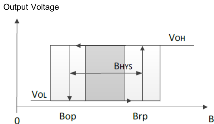
Output behavior of CYD511
